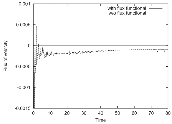
Figure 8: Time history of flux of velocity through the interface(Case B1 and B2).
