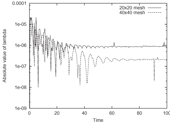
Figure 10: Time history of Lagrange multiplier |\lambda_h| (Case A1 and A3).
