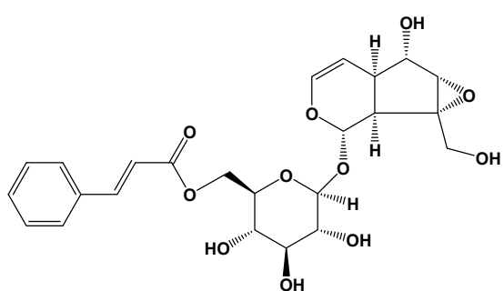
picroside I
