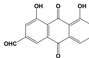
rheinal
