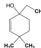
patchouli alcohol
