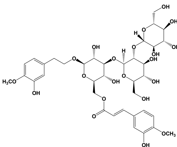
scroside A
