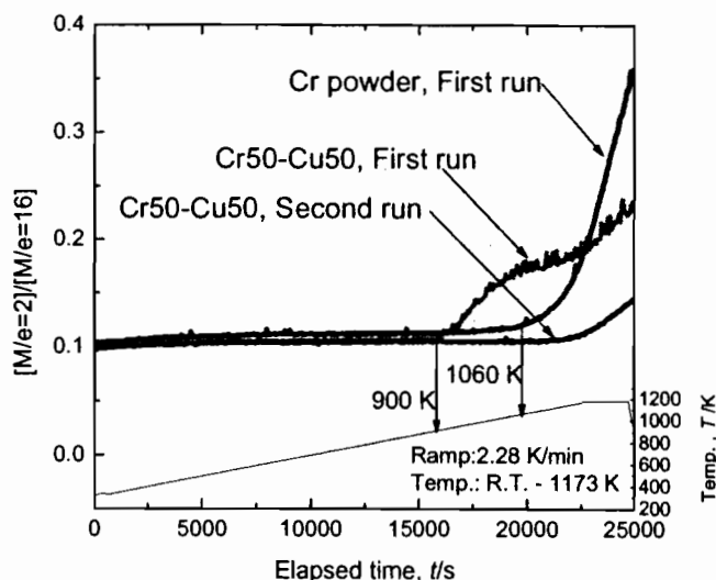
Fig. 2. Thermal decomposition of methane by pure Cr and Cr-Cu alloy.
