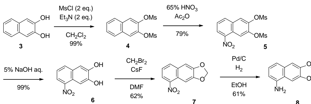
Scheme 1. Preparation of 1-Naphthylamine
